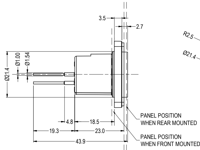
SUPPLIED WITH GASKET CP30060SA3
