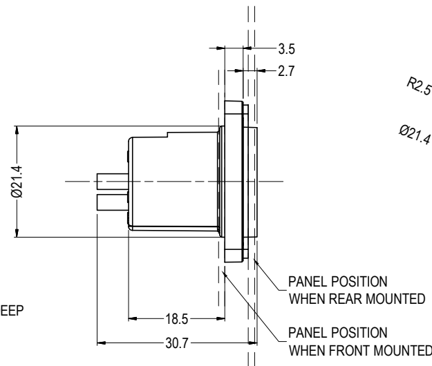
SUPPLIED WITH GASKET CP30060SA3
