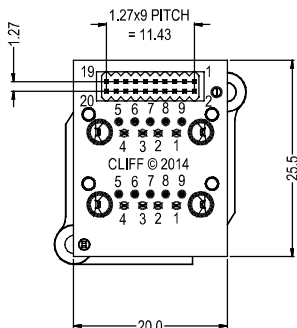
PART No. CP30097
