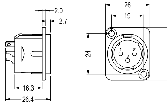
FC61905 - XLR SOCKET MALE 3DCM/BM Scale 2x1
