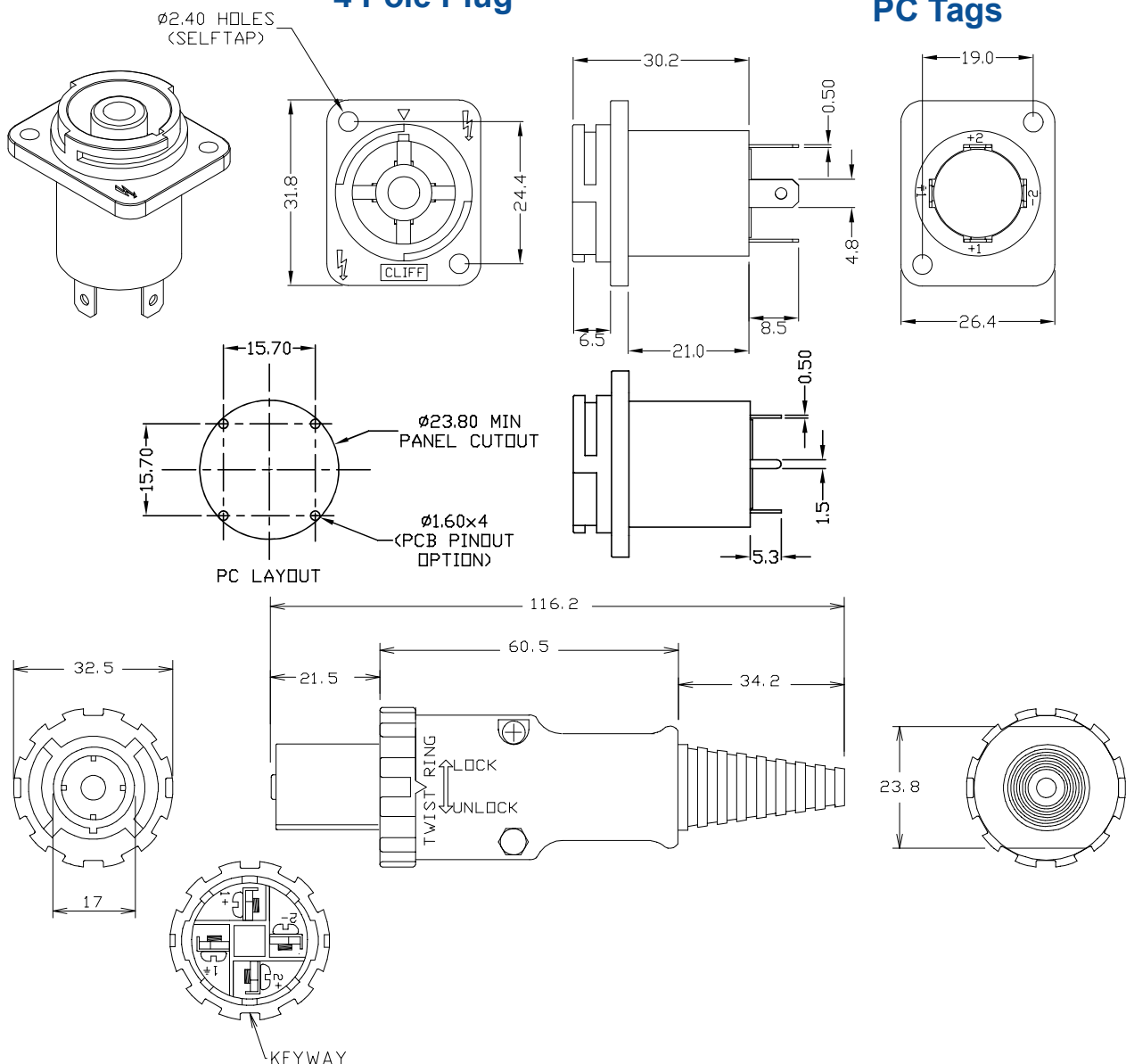
FCR2062 4 Pole Plug
