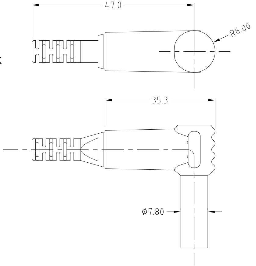
FCR6341B - 90° PLUG P149XR BLACK
